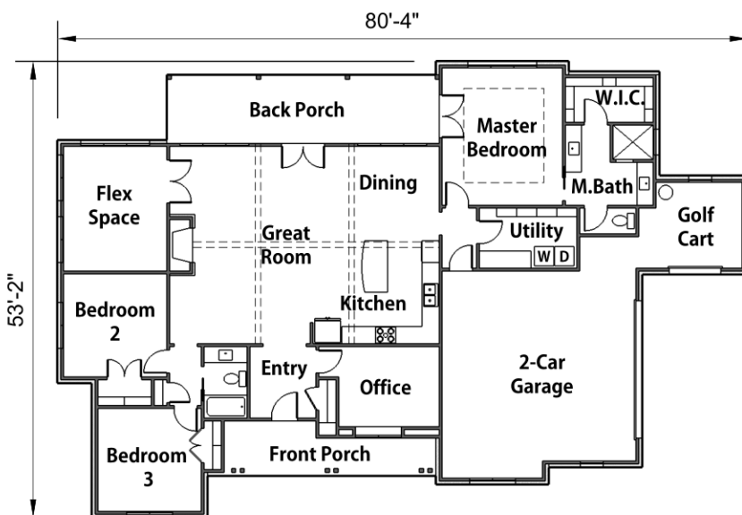
Floor Plan
